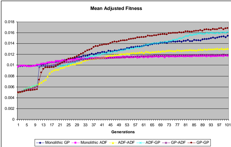
Figure 1. Mean adjusted fitness (10 replications) – higher is better
