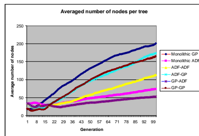
Figure 2. Average tree size (10 reps)
