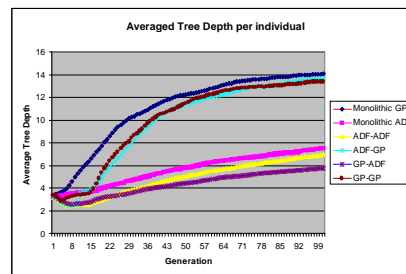
Figure 3. Max tree depth (10 reps)
