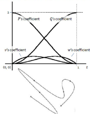
Polynomial weighting functions in Hermite curve equation
