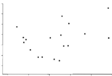
Conventional Scatterplot
