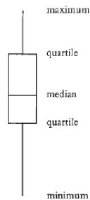
and John Tukey's "box plot"
