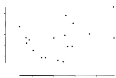
Conventional Scatterplot
