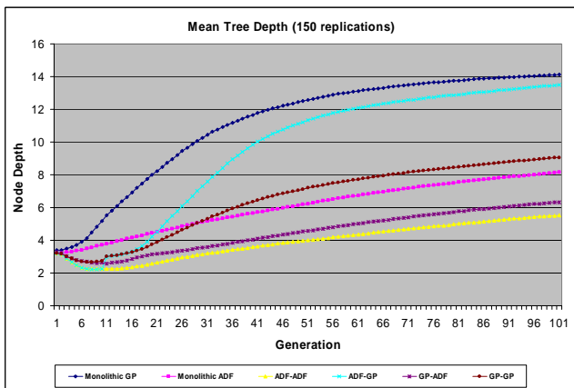
Figure 3. Mean tree depth in each generation (averaged over 150 reps)
