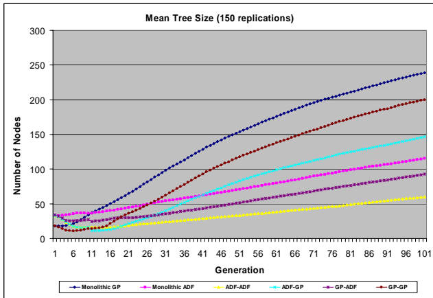
Figure 2. Mean tree size in each generation (averaged over 150 reps)
