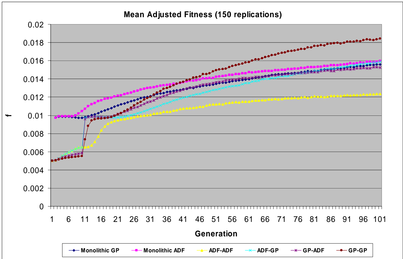
Figure 1. Mean adjusted fitness in each generation (averaged over 150 replications) – higher is better.
